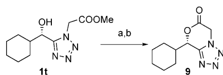
Scheme 3. Lactonization of dipeptide mimic 1t : a) potassium hydroxide, methanol, room temperature, 6 h; b) dicyclohexylcarbodiimide/4-dimethylaminopyridine, N,N -dimethylformamide/dichloromethane, room temperature, 24 h, 82%.
